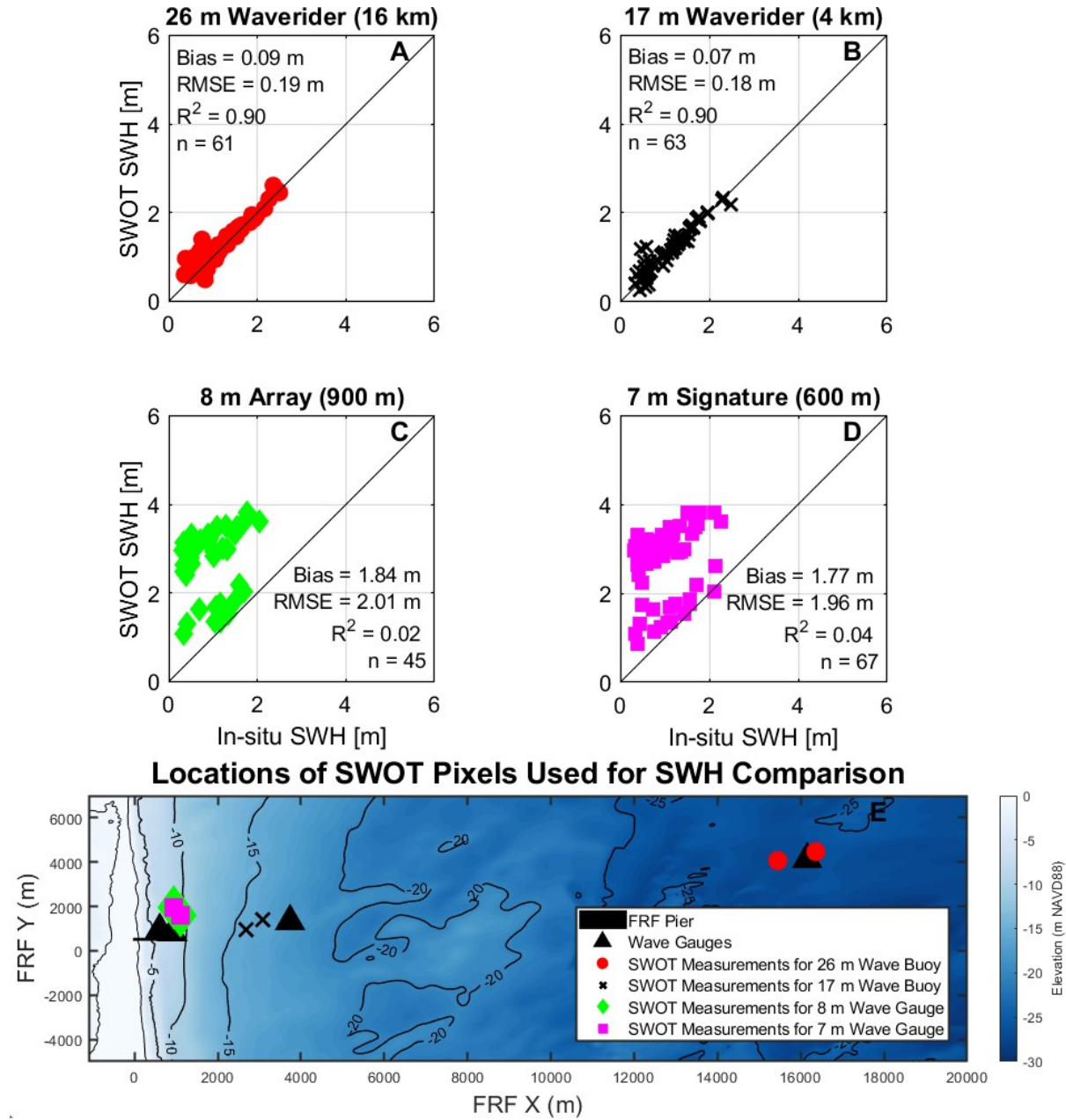
Figure 3. SWOT Significant wave height (SWH) estimates (y axis) vs. in-situ SWH measurements (x axis) at (a) Waverider buoy in 26 m water depth (16 km offshore), (b) waverider buoy in 17 m
