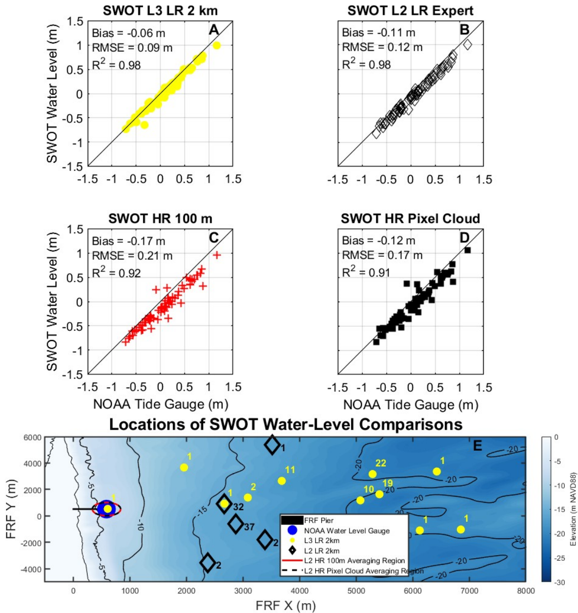
205 206 Figure 2. SWOT WSE (y axis) vs. NOAA Tide Gauge Water Level Measurement (x axis) for (a) SWOT 207 Level 3 LR SSH Expert (2 km), (b) SWOT Level 2 LR SSH Expert (2 km), (c) SWOT Level 2 HR 100m 208 Raster, and (d) SWOT Level 2 HR Pixel Cloud and the e) locations of SWOT measurements used for
