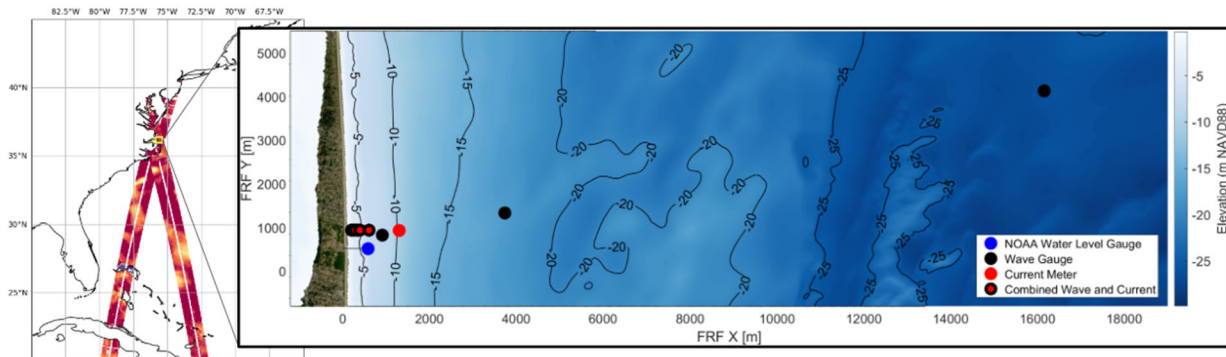
Figure 1. Map of the East Coast of the United States with SWOT passes 63 and 354 showing L3 LR SSH Unsmoothed sea surface height anomaly (SSHA) with the Field Research Facility (FRF) called out on the right showing the research pier (solid black line), NOAA tide gauge (blue circle), and y=940 m transect of wave gauges (black circles). The color bar shows water depth (NAVD88) with 5 m depth contours
